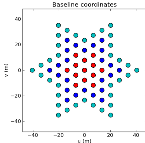
Figure 2 – Fourier plane (" u - v ") coverage of the MROI for an object at the zenith. Coverage for arrays with 4, 7, and 10 telescopes is indicated by the color codes of the dots (all arrays include the coverage of smaller arrays as subsets).
